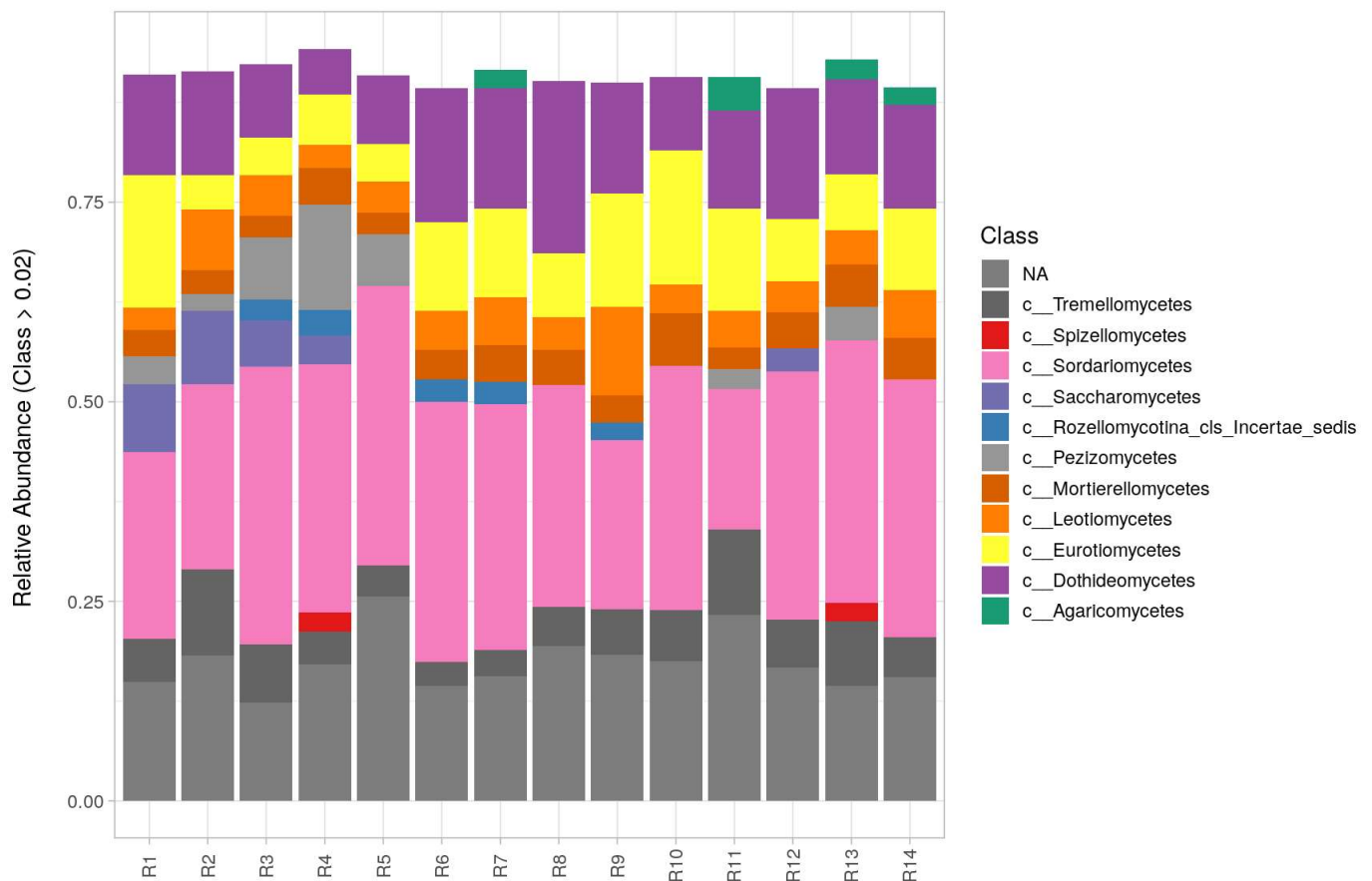
Fungal communities by sample at class level Relative abundance
