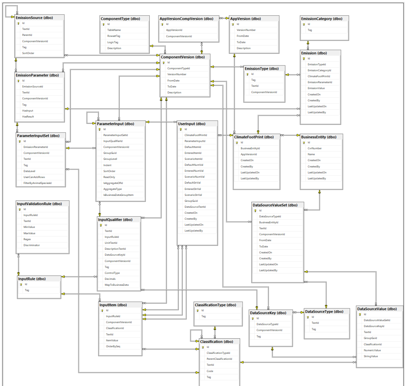
Figur 1. Datamodel
